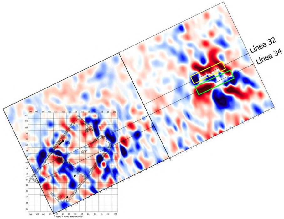
Figure 13. Georadar verification of magnetic anomalies.
