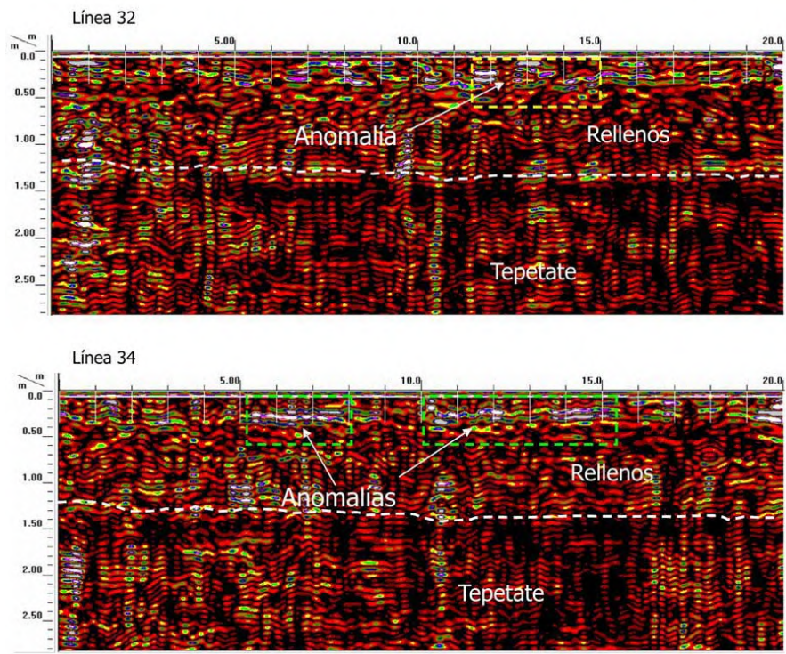
Figure 14. Radargrams of the circular anomaly.
