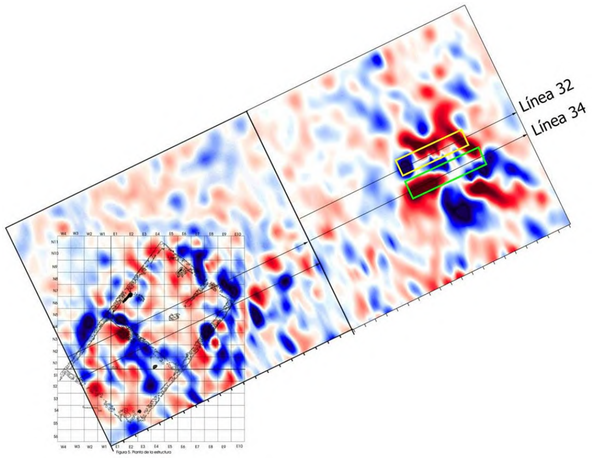
Figure 15. Radar verification lines.
